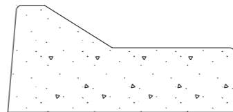
SECTION 5 NOT TO SCALE
