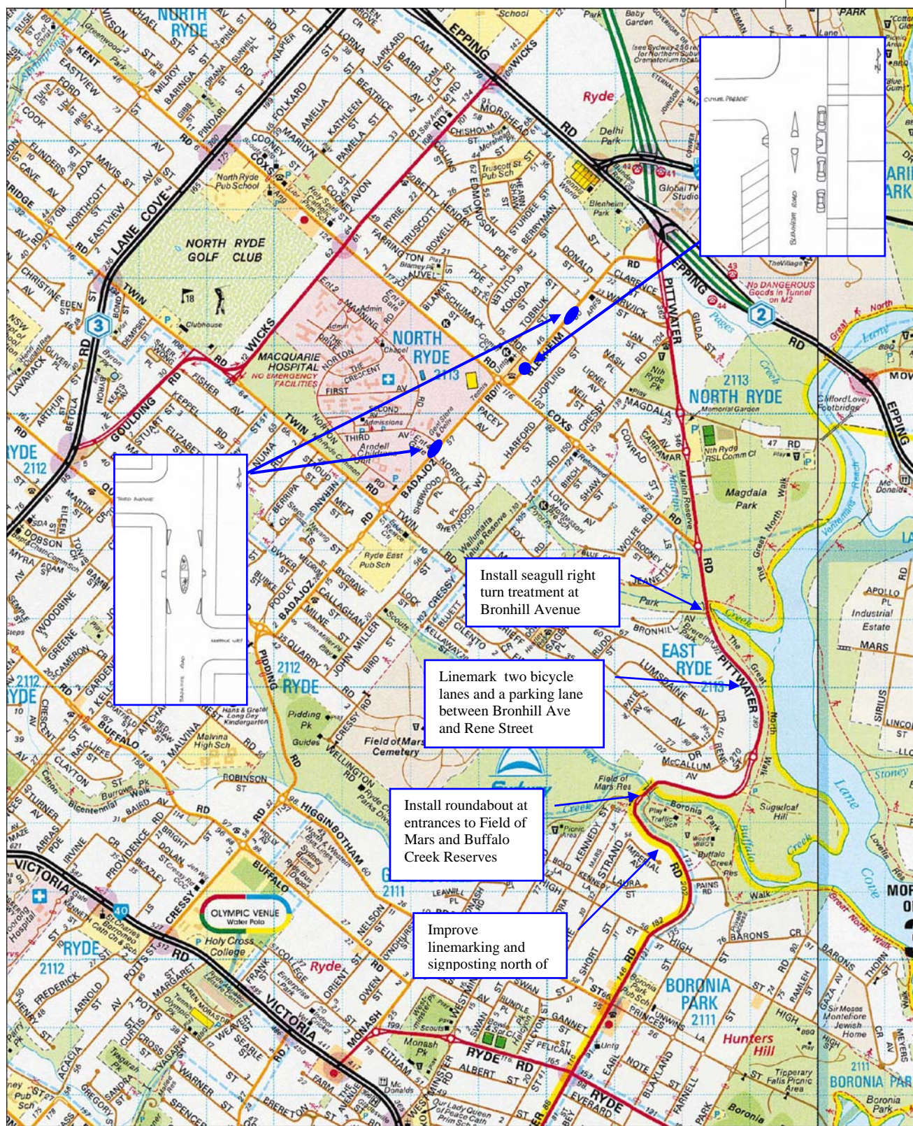
Figure 1: Draft Traffic Management Devices
