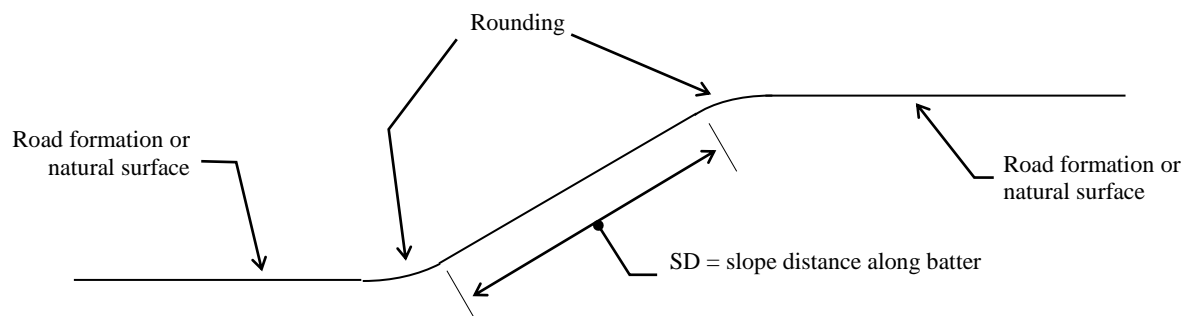
Figure G71.1 – Rounding at top and bottom of batter planes
