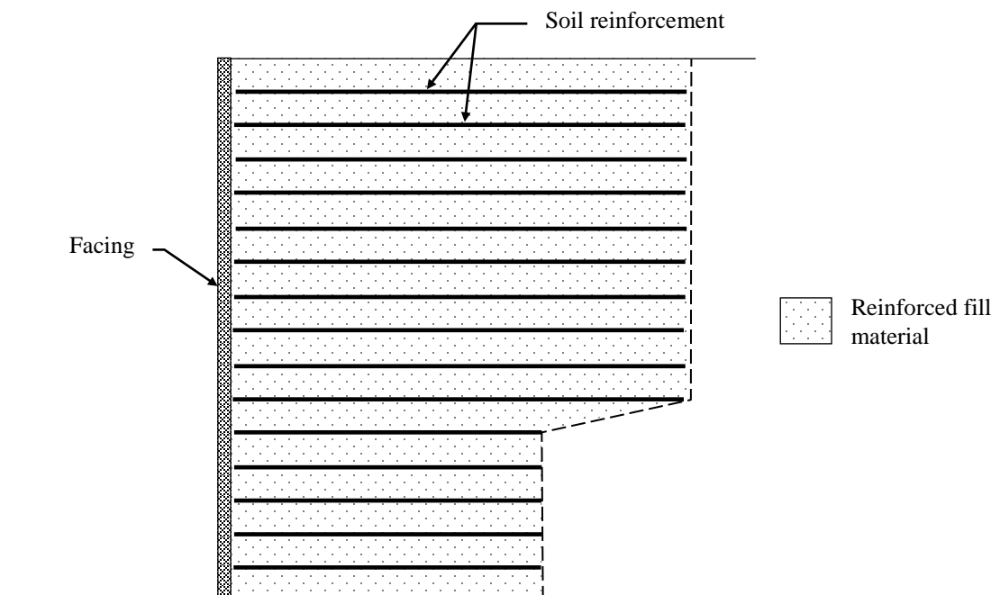
Figure R59.1 - Extent of Reinforced Fill Material for Payment Purpose
