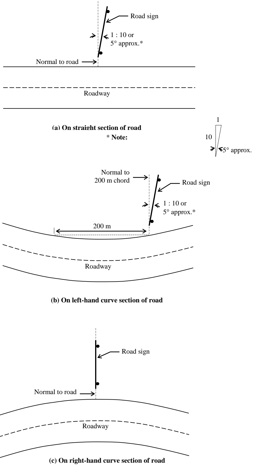
Figure R143.1 – Sign Orientation on Straight Sections and Curved Sections of Road
