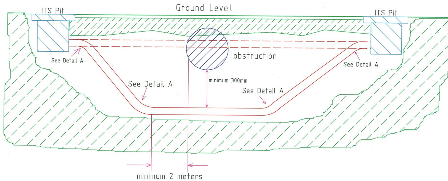
Diversion of Underground Cableway in vertical plane.
