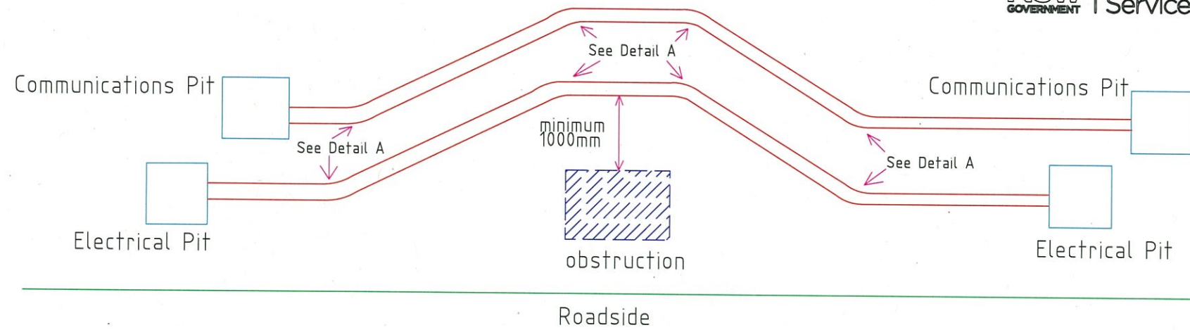
Diversion of Underground Cableway in horizontal plane.
