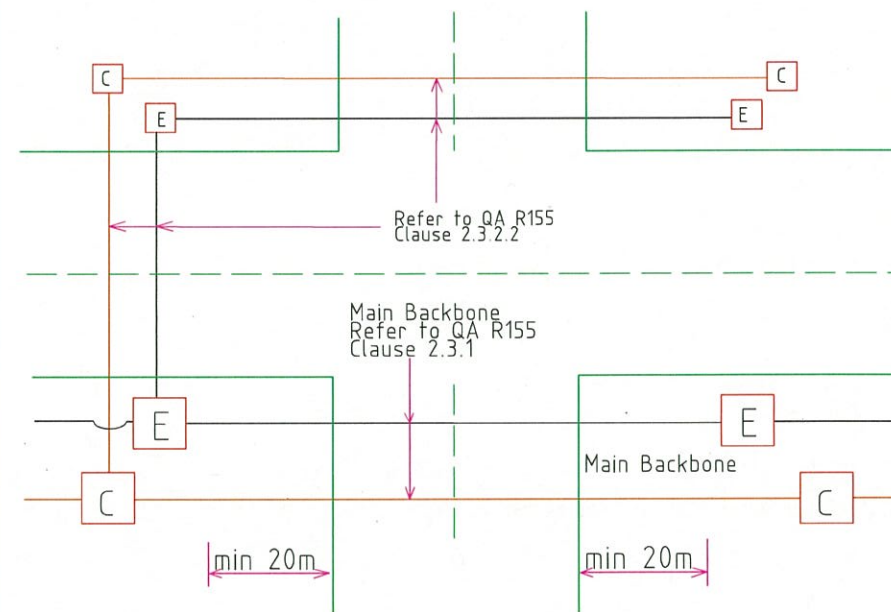
Fourway intersection without Traffic Control Signal(TCS)
