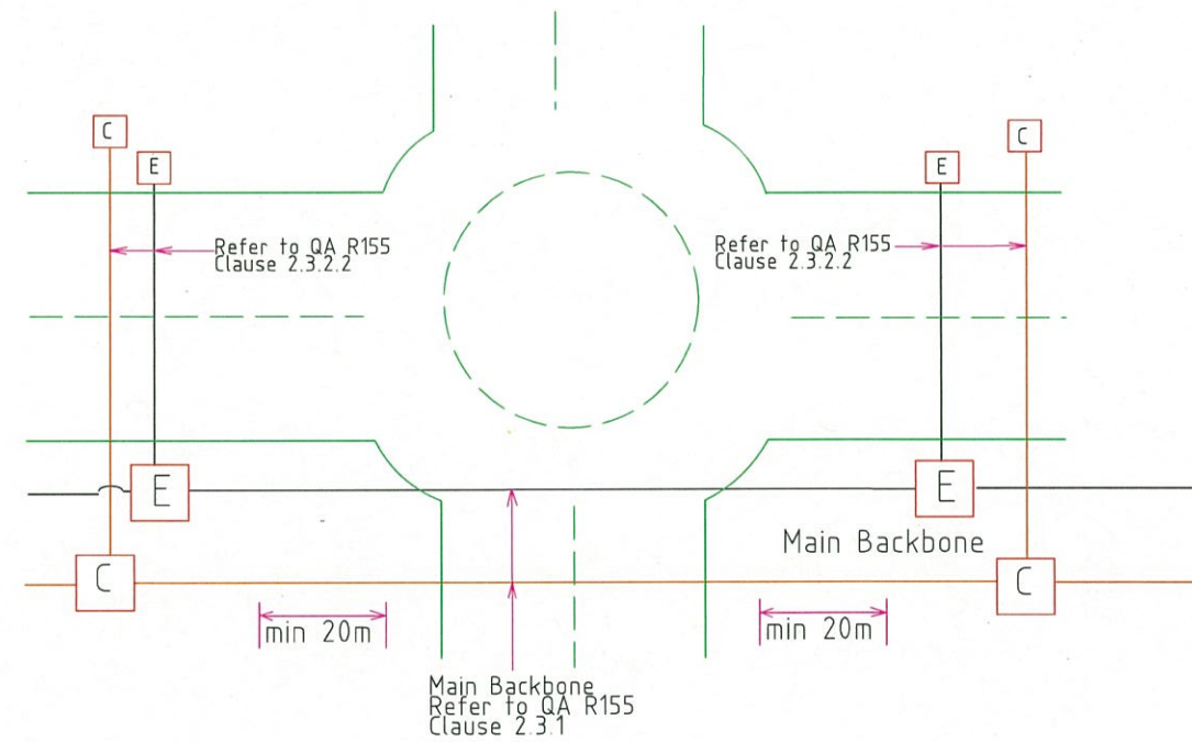
Roundabouts without Traffic Control Signal(TCS)
