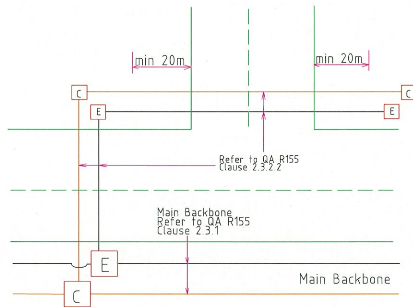
T Junction without Traffic Control Signal(TCS) (Main Backbone below side road)
