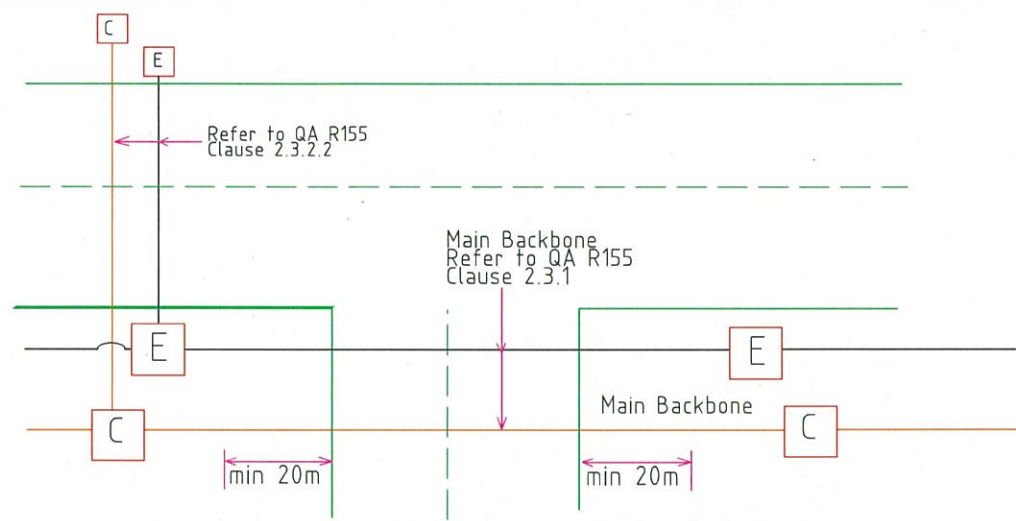
T Junction without Traffic Control Signal(TCS) (Main Backbone opposite side road)
