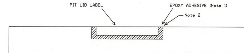
CROSS SECTIONAL SIDE VIEW OF PIT LID WITH LABEL (Not to scale)
