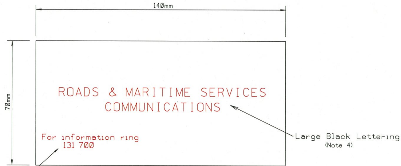
COMMUNICATIONS PIT LID LABEL (See Note 1)
