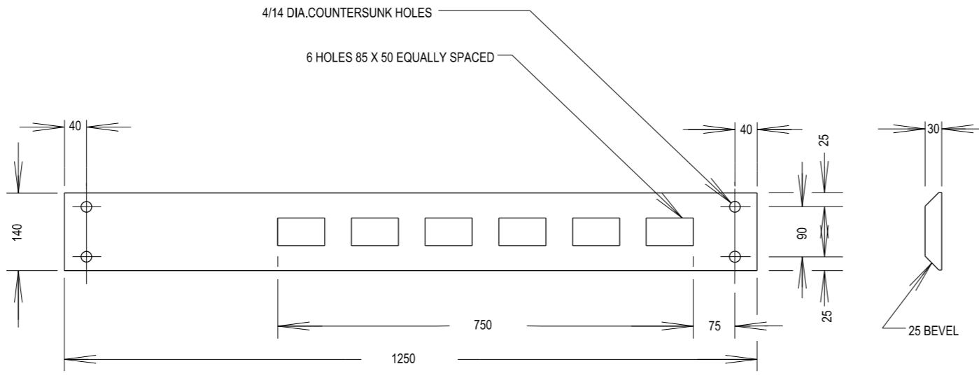
MILD STEEL GRILLE 1 REQUIRED
