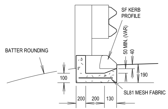
SECTION 3 NOT TO SCALE
