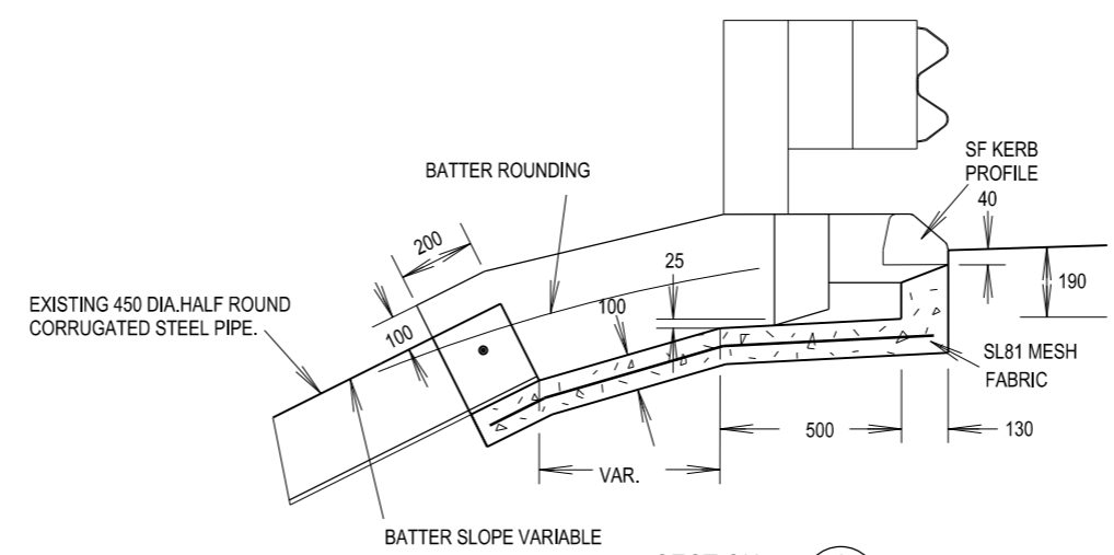
SECTION 2 NOT TO SCALE
