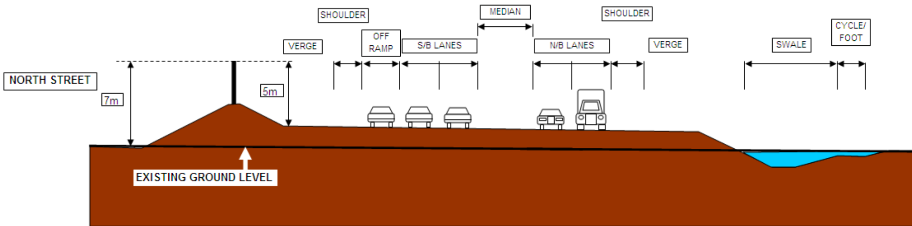
SECTION THROUGH CURRENT HIGHWAY ALIGNMENT BETWEEN EDWARD & ALBANY STREETS
